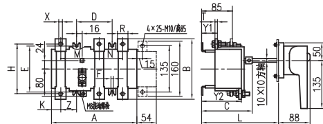
HH15P (QP) -630, 1000A
