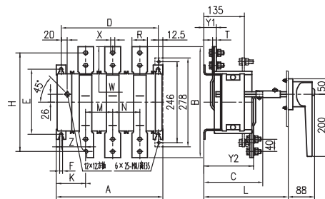
HH15P (QP) -1250, 1600A
